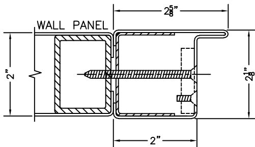
2" MODULAR WALL
