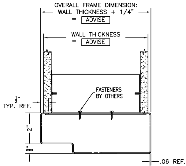
JAMB PROFILE, SLIDE-IN S/S FRAME
