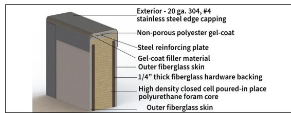
Molded Fiberglass Construction Our exclusive process utilizing polyester gel-coat, offers a fiberglass door that is truly seamless. Cleanseal fiberglass doors are built to a higher standard so they withstand the harshest conditions and still look great year after year.
