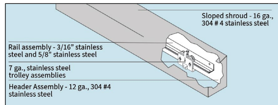
*Standard Header and Rail Assembly For superior cleanability, durability and aesthetic appeal
