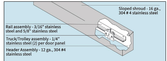
*Standard Header and Rail Assembly For superior cleanability, durability and aesthetic appeal
