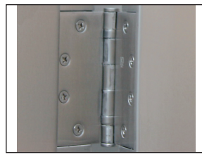
Fully Mortised Hinges (Shown on stainless steel door) Flush mortised hinges provide a clean and smooth finish to the door.
