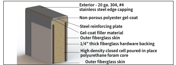
Molded Fiberglass Construction Our exclusive process utilizing polyester gel-coat, offers a fiberglass door that is truly seamless. Cleanseal fiberglass doors are built to a higher standard so they withstand the harshest conditions and still look great year after year.
