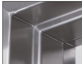
Frame Assembly Fully mitered and completely welded through the throat. Single or double rabbet
