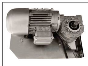
Direct Shaft Drive High speed opening up to 100"/sec. High performance AC drive and absolute encoder controlled.
