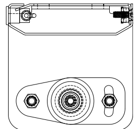
LH Slide Trail Edge Face Frame Top View
