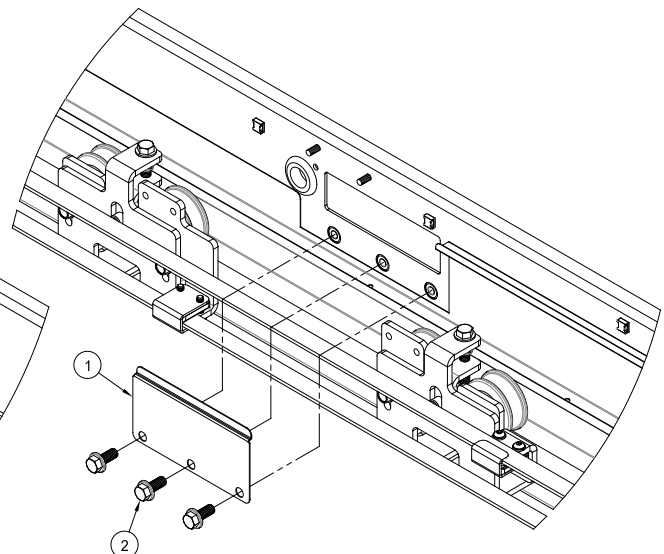
PWR BI-PART, NO BOLT LOCK OPTION (F3)
