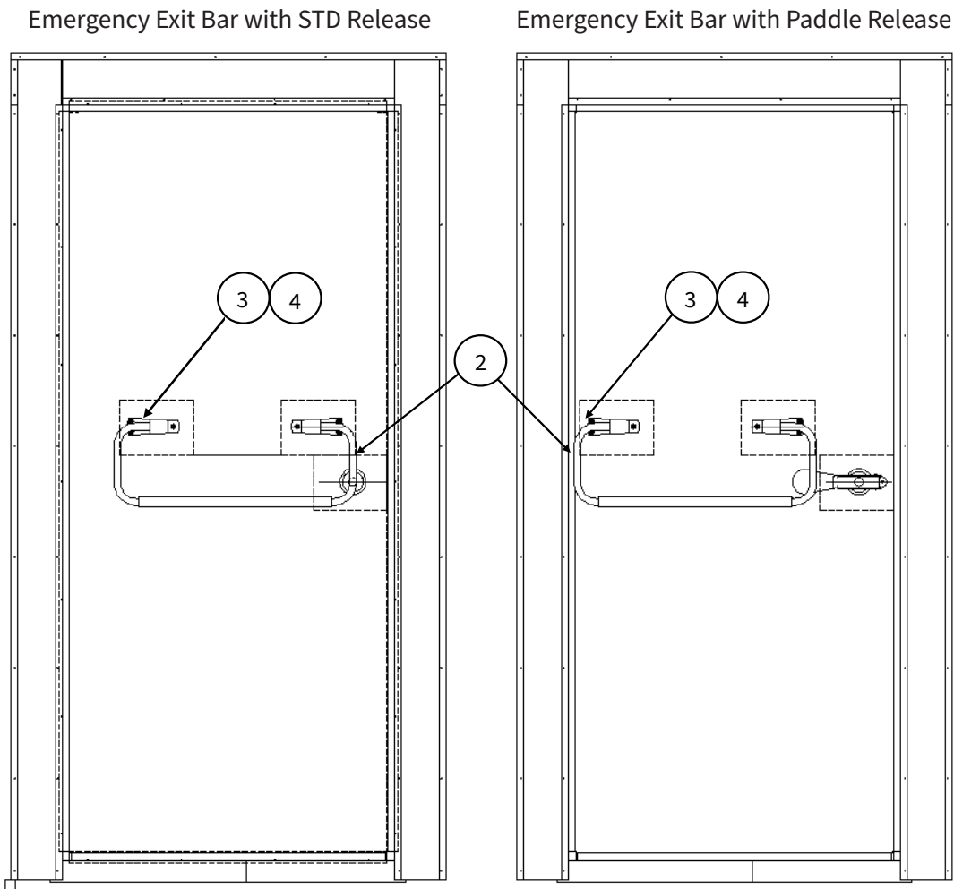
Figure 14: Optional Emergency Exit Devices
